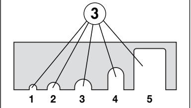
Flat development of the internal (1) pre-setting device
